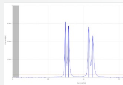
Signal with multi-layer thickness measurements (max. 6 peaks)
