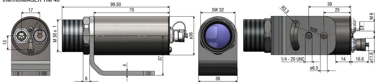
thermoIMAGER TIM 40
