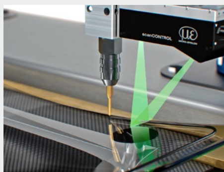
In-line inspection of adhesive bonding
