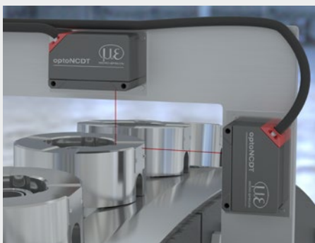
Dimension control of turned parts
