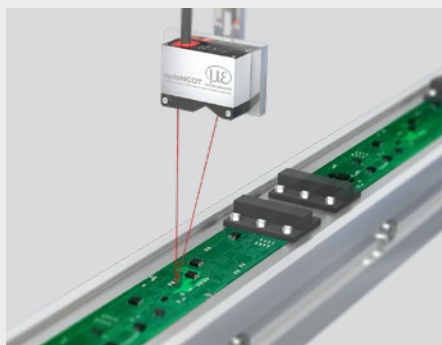
Use in PCB assembly
